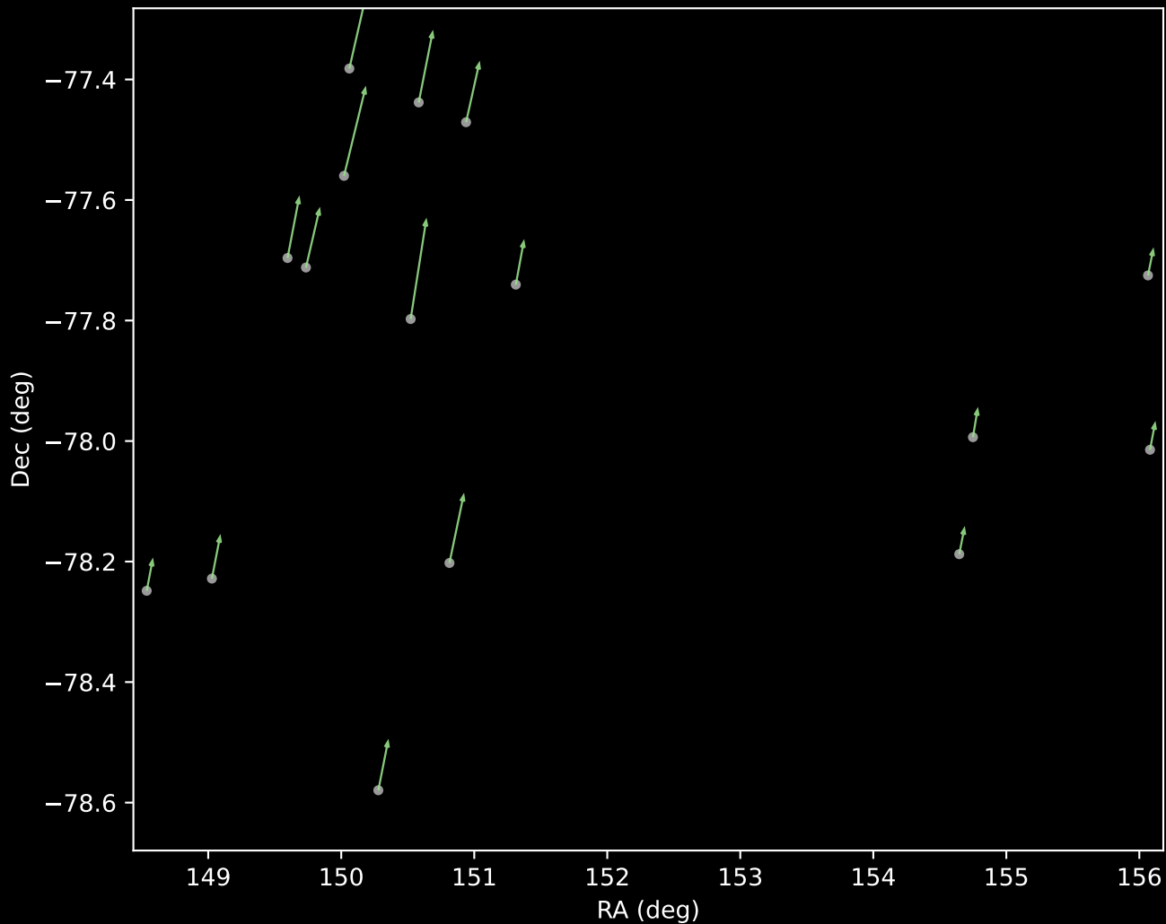
GALAH DR4 Cluster 5 Proper Motion Vectors (n=16)
