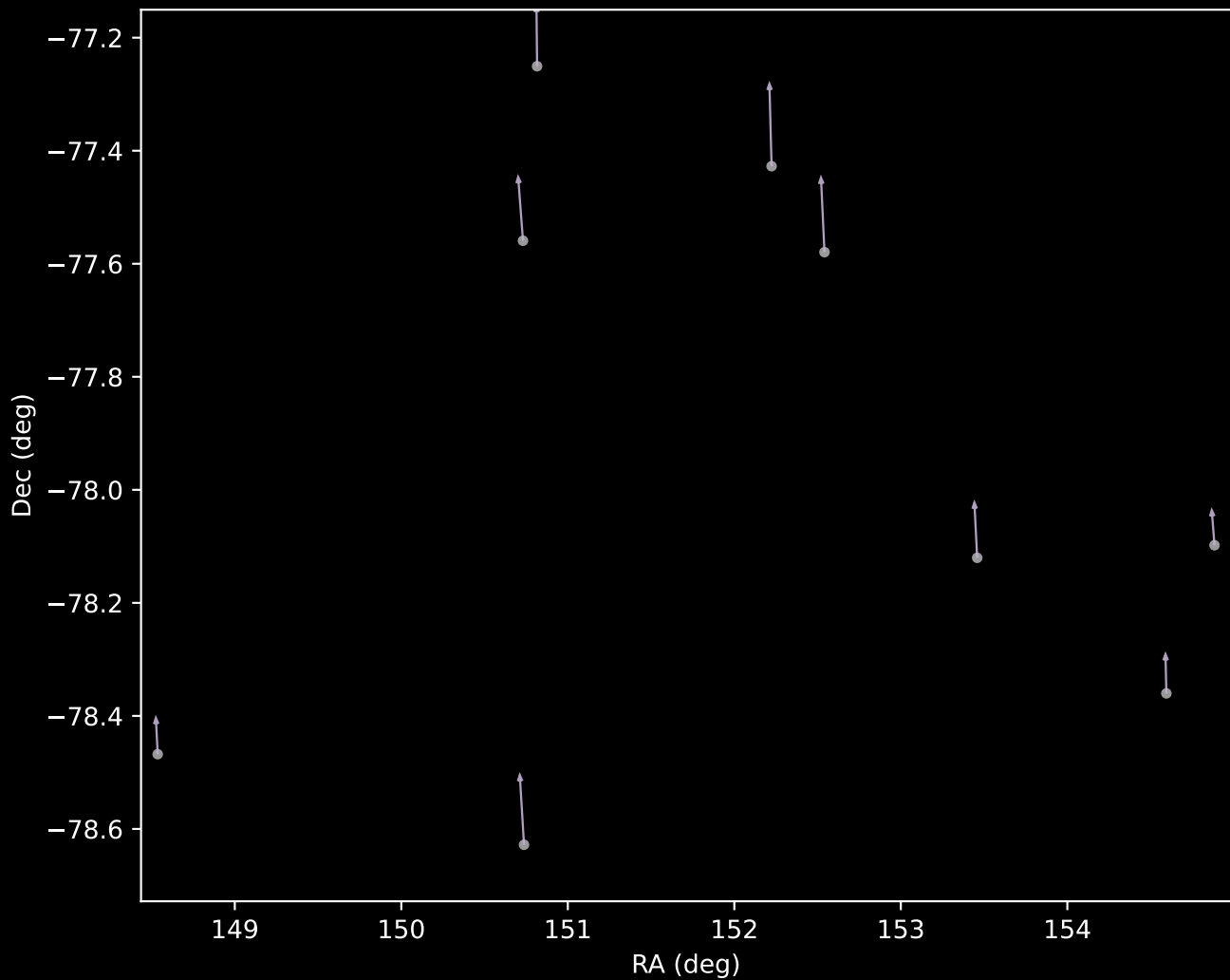
GALAH DR4 Cluster 9 Proper Motion Vectors (n=9)
