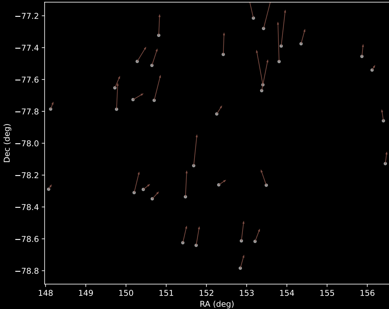
GALAH DR4 Cluster 10 Proper Motion Vectors (n=34)
