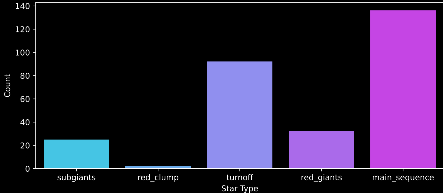
GALAH DR4 Field: [410] Count plot of Star Type
