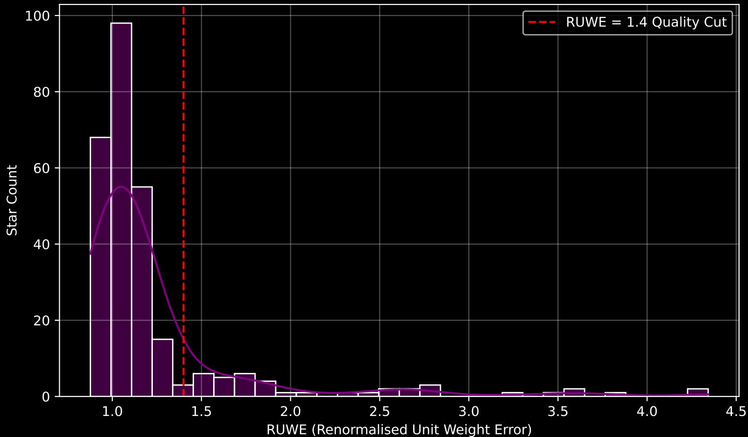
GALAH DR4 Field [410] RUWE Distribution (n= 278)
